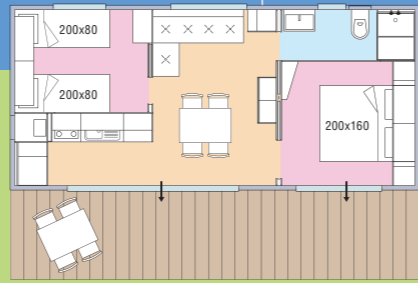
RIVER LODGE 4 34.4 m 2 + 20.6 m 2 Terrasse max. 4 Personen, min. 2 Person Nr. 426, 427, 428, 429, 430, 431, 432, 439, 441, 443
